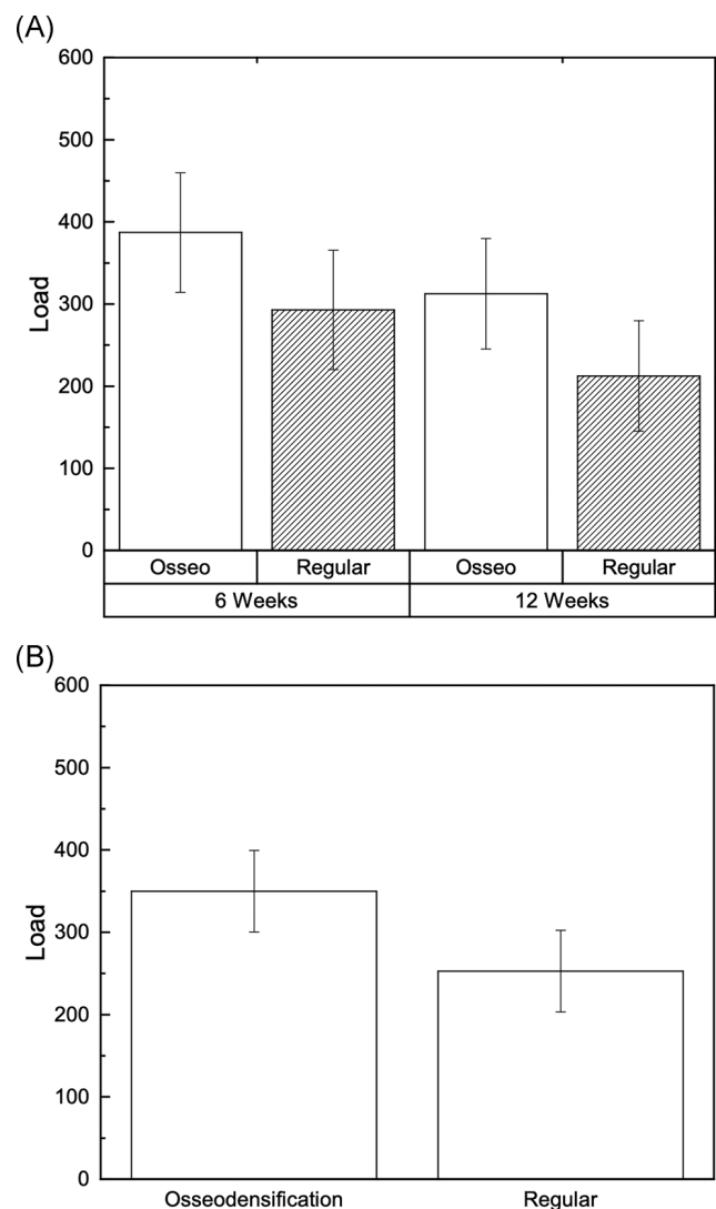
FIGURE 4 Bar graphs presenting the mean removal load (N) ± 95% CI of (A) as function of time and instrumentation, where OD group show significantly greater load bearing capability as compared to the R group at both 6- and 12-week. And (B) mean peak load with corresponding 95% CI independent of time. Letters denote statically homogenous groups. CI, confidence interval; OD, osseodensification; R, regular
